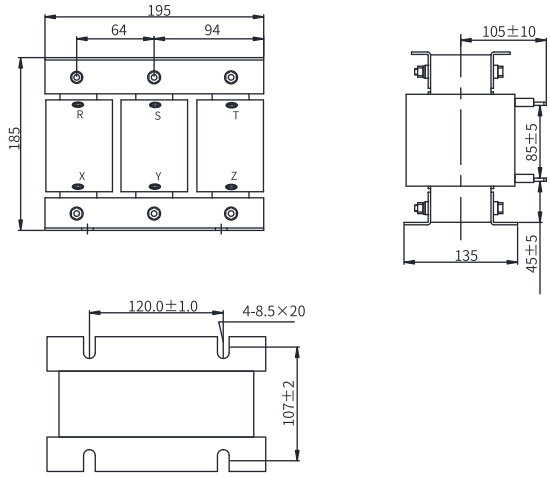
Figure 4-4 Dimensions of 50 A AC input reactor
