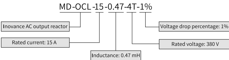
Figure 4-13 AC output reactor model
