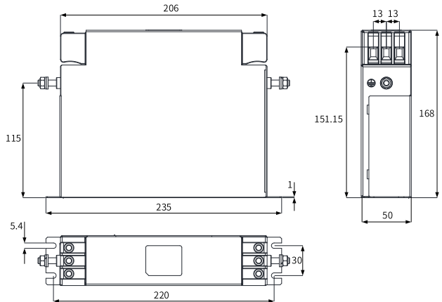
Figure 4-9 Filter dimensions (FN3288-40-33) (unit: mm)
