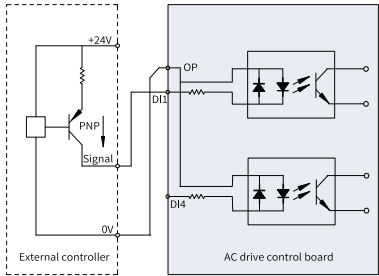
Source wiring using external 24 V power supply
