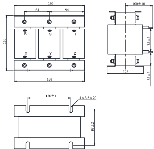
Figure 4-2 Dimensions of 15 A AC input reactor
