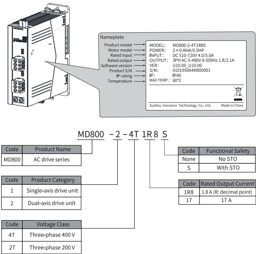
Figure 1-2 Nameplate and model number of the drive unit
