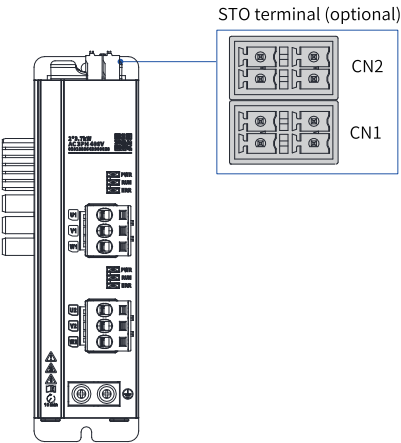
Figure 3-7 Arrangement of STO terminals of drive unit (dual-axis)
