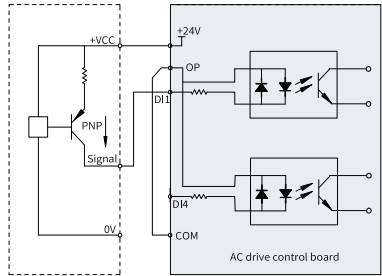
Source wiring using internal 24 V power supply of the AC drive
