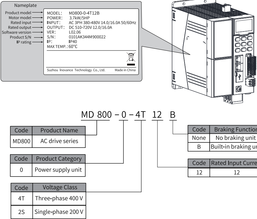
Figure 1-1 Nameplate and model number of the power supply unit
