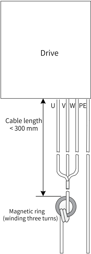
Figure 5-2 Installing a magnetic ring
