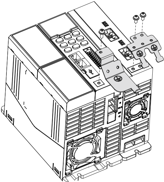
Figure 4-24 Mounting position of the shielding bracket
