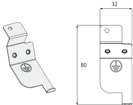
Figure 4-22 Dimensions of EMC shielding bracket for the power supply unit
