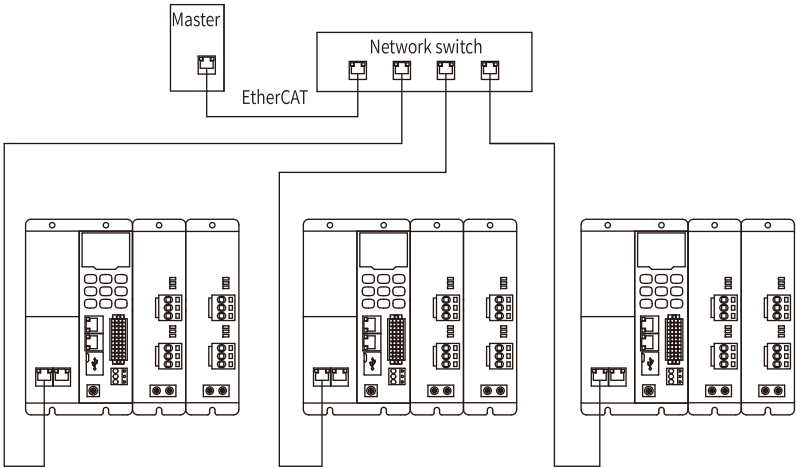
Figure 3-28 EtherCAT star topology
