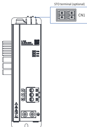
Figure 3-6 Arrangement of STO terminals of drive unit (single-axis)
