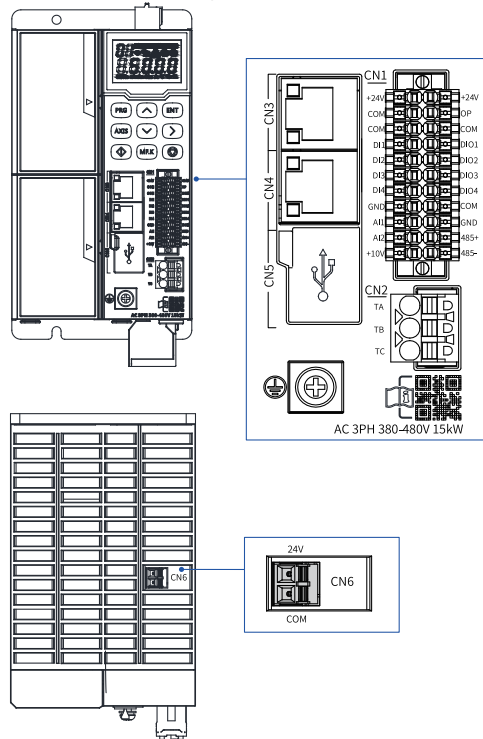
Figure 3-5 Arrangement of control circuit terminals of power supply unit
